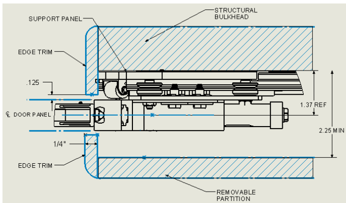
3519-172-1 MECHANICAL DOOR PLAN VIEW
